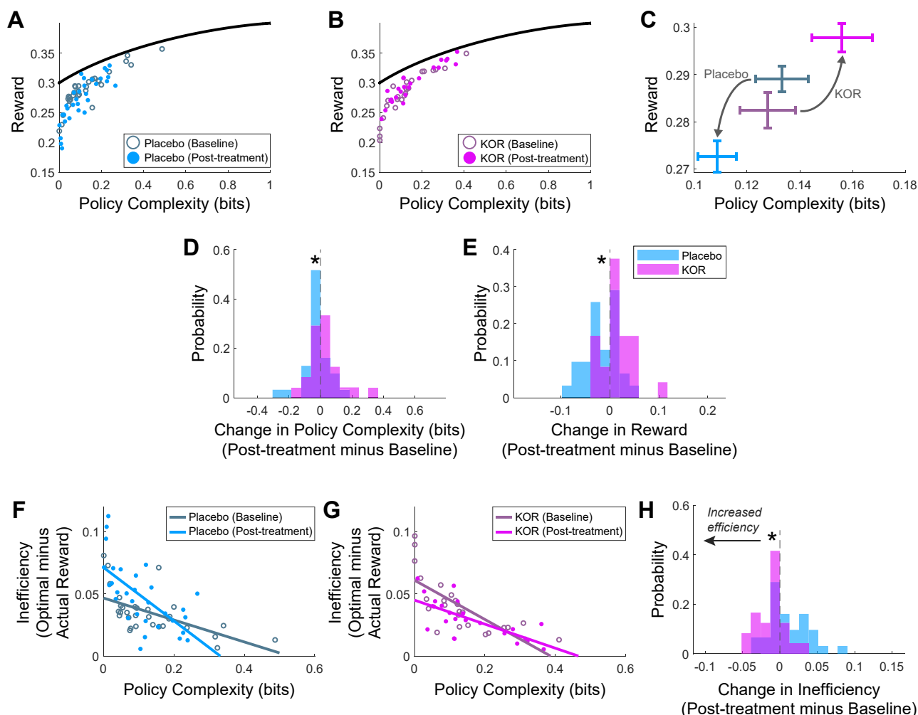
Figure 2. Changes in policy complexity and efficiency as a function of kappa opioid receptor (KOR) antagonism. ( A, B ) Reward-complexity relationship for the placebo and KOR groups at baseline and post-treatment. The black line shows the reward-complexity frontier, which indicates the optimal reward as a function of policy complexity. ( C ) Mean \pm SEM reward-complexity relationship as a function of treatment (placebo or KOR antagonism) and time (baseline or post-treatment). ( D ) Change in policy complexity (post-treatment minus baseline) as a function of treatment. ( E ) Change in reward (post-treatment minus baseline) as a function of treatment. ( F, G ) Relationship between inefficiency and complexity for the placebo and KOR groups. Overlaid lines are from a linear mixed-effects model fitting inefficiency as a function of policy complexity, treatment, and time. ( H ) Change in inefficiency (post-treatment minus baseline) as a function of treatment. * p < .05 .
