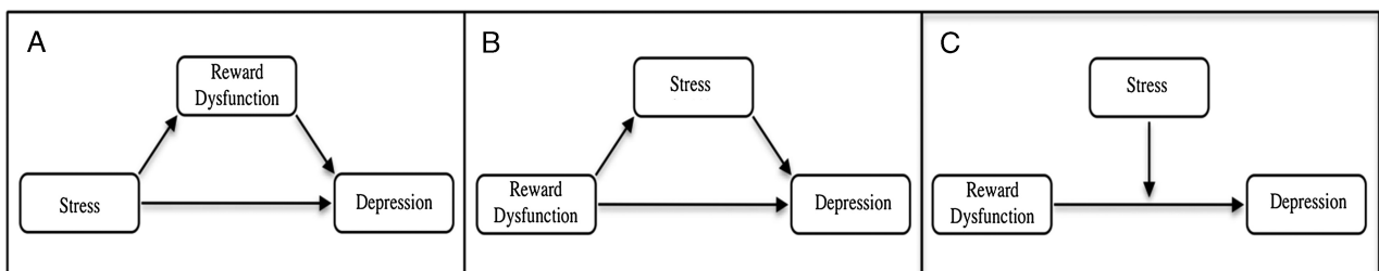
Figure 1. Examining the relationship among stress, reward dysfunction, and depression. (A) reward mediation model; (B) stress generation model; (C) titration model.
